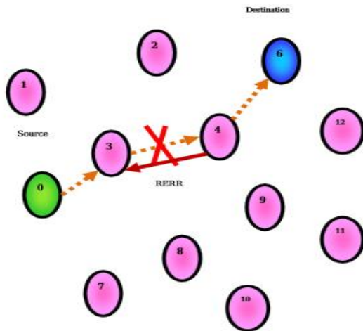
Fig.6 Link failure occur at the middle of transmission.
