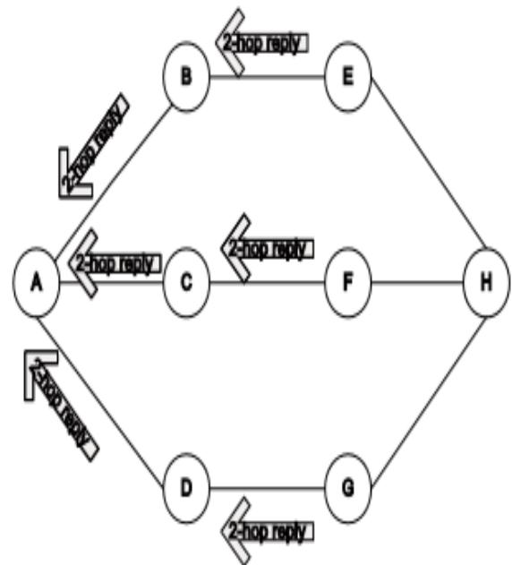
Fig. 2. E, F, and G send 2-hop reply to A through B, C, and D.
